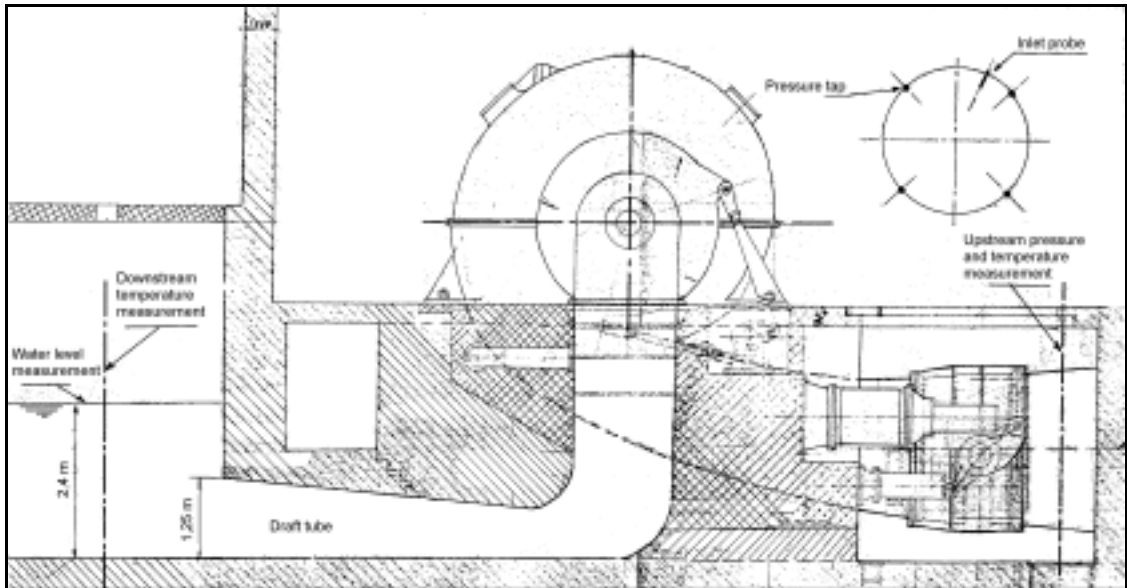
Figure 8 - Pégage de Vizille power plant - Measurement device
