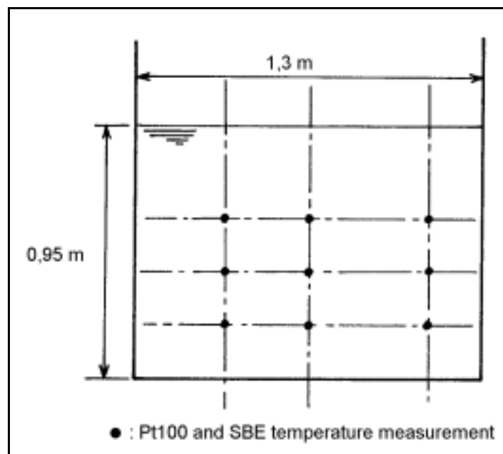
Figure 5 - Migoelou power plant - Measurement device
