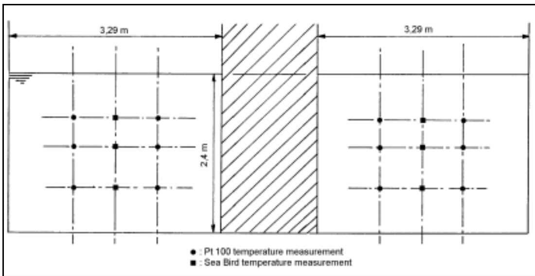
Figure 9 - Pégage de Vizille power plant Temperature measurement at the draft tube outlet
