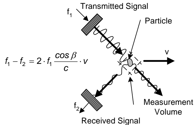
Figure 2. Acoustic Doppler velocimetry (ADV)
