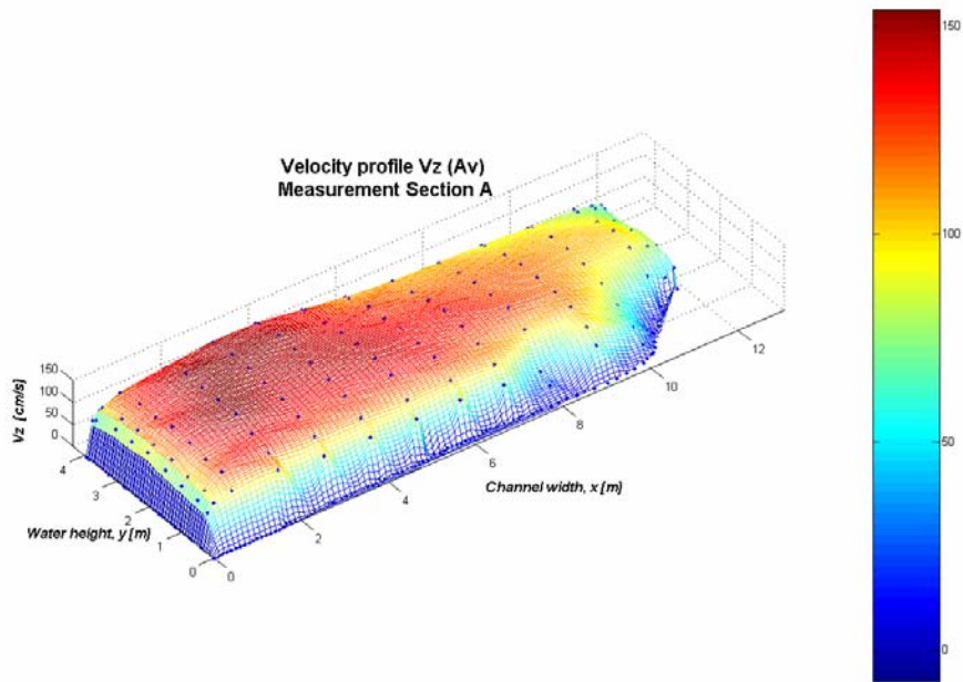
Figure 11. Time averaged distribution of velocity v_z , measured with ADV in cross section A
