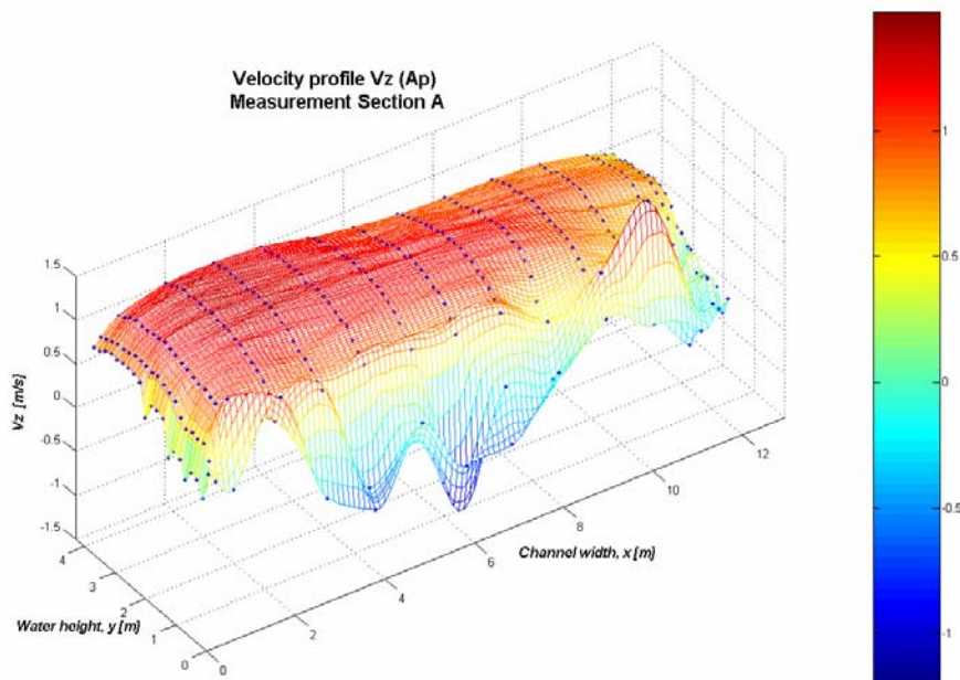
Figure 12. Time averaged distribution of velocity v_z , measured with ADP in cross section A: the data shown in the vicinity of the boundaries are affected by acoustic reflections.
