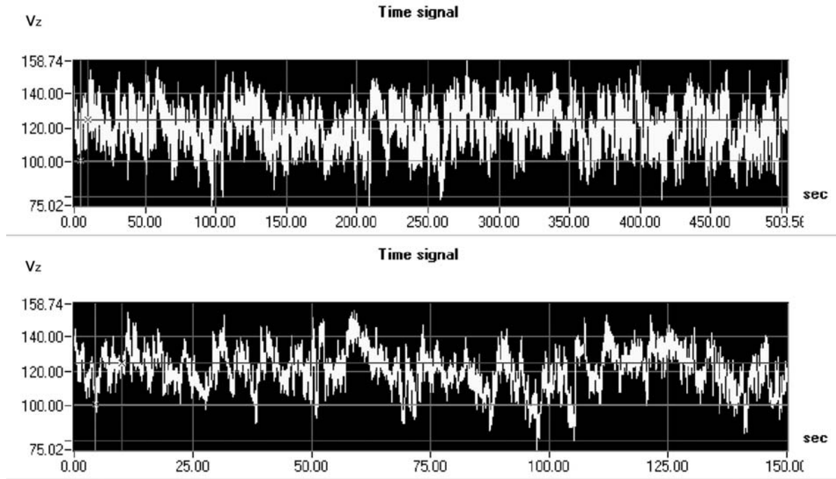
Figure 9. Typical acquired time signal measured with the ADV probe (velocity in cm/s).
