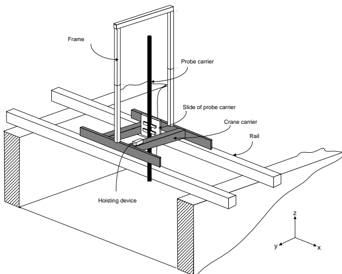
Figure 7. Setup of measurement
