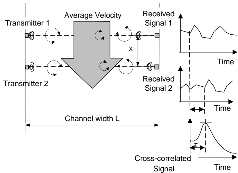
Figure 4. Scintillation method
