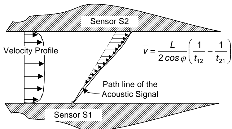
Figure 1. Acoustic transit time measurement
