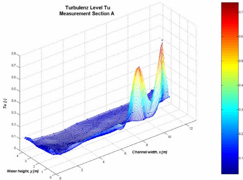
Figure 10. Turbulence level distribution measured with ADV in cross section A
