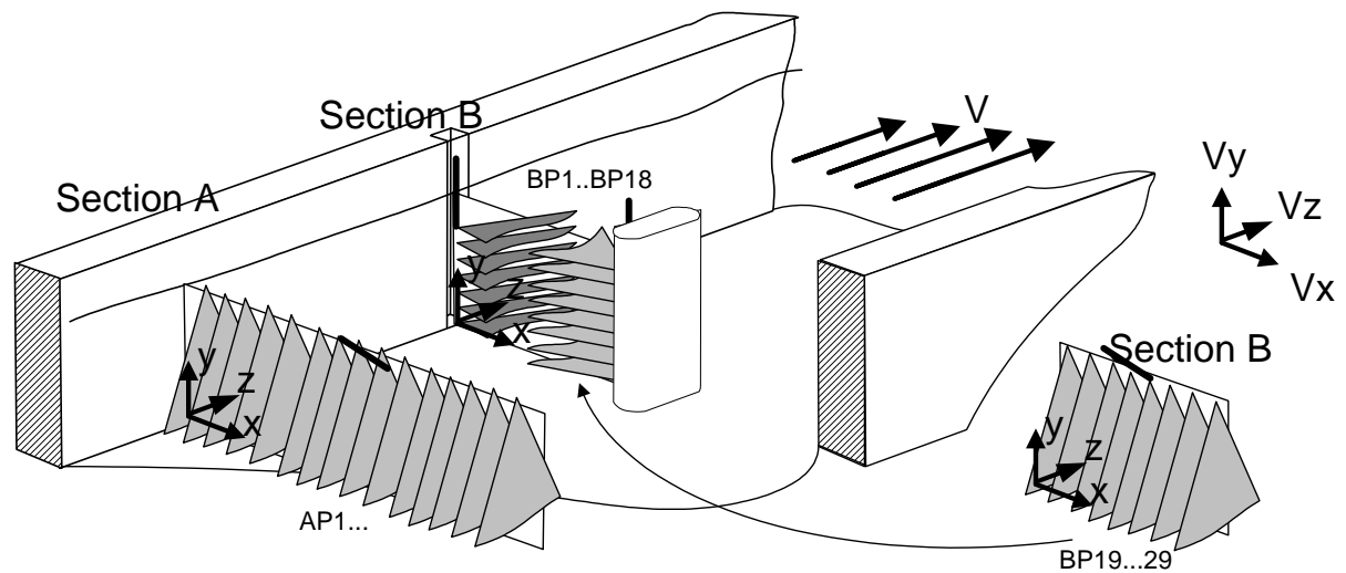
Figure 8. Measuring cross sections and orientation of the acoustic beams of the ADP
