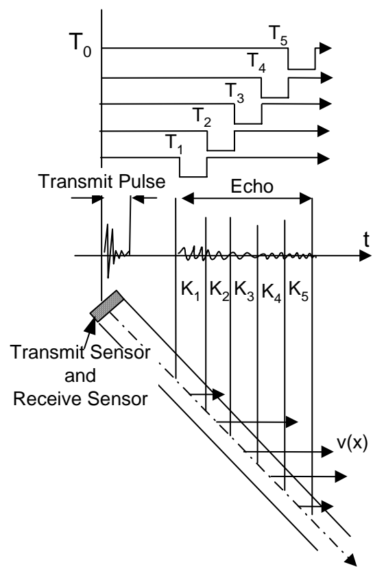
Figure 3. Acoustic Doppler Profiler (ADP)
